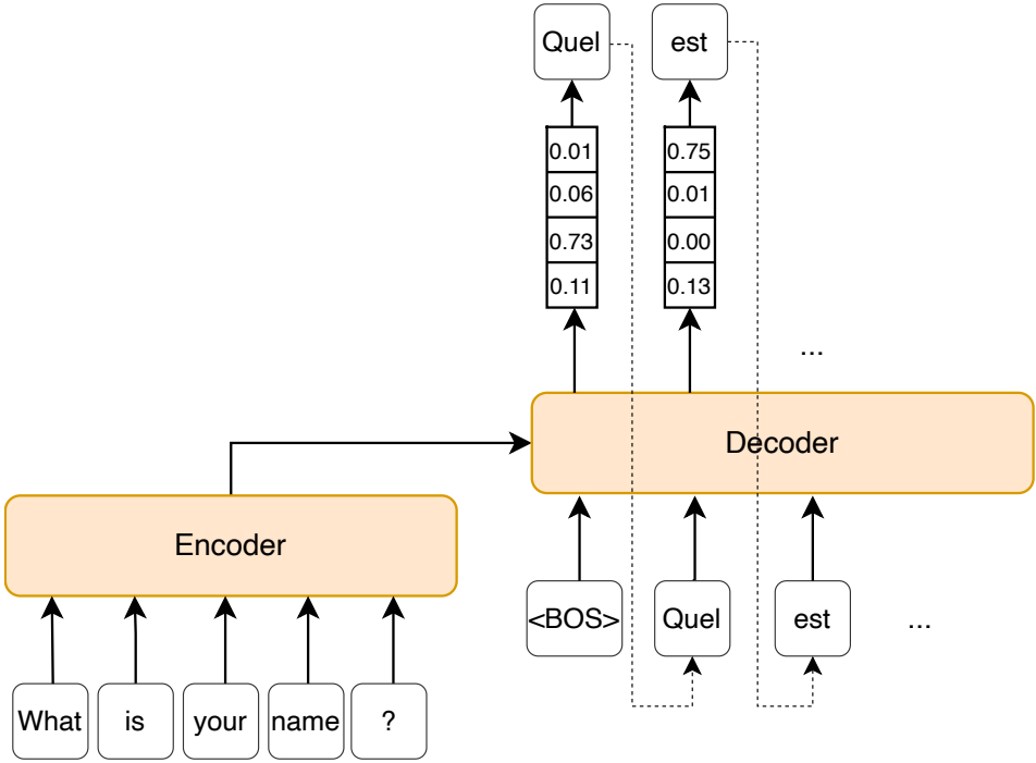
Figure 22: Generating translation
