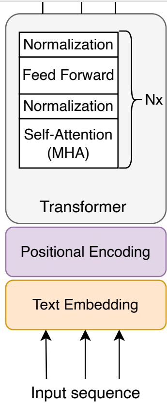
Figure 12: Encoder components
