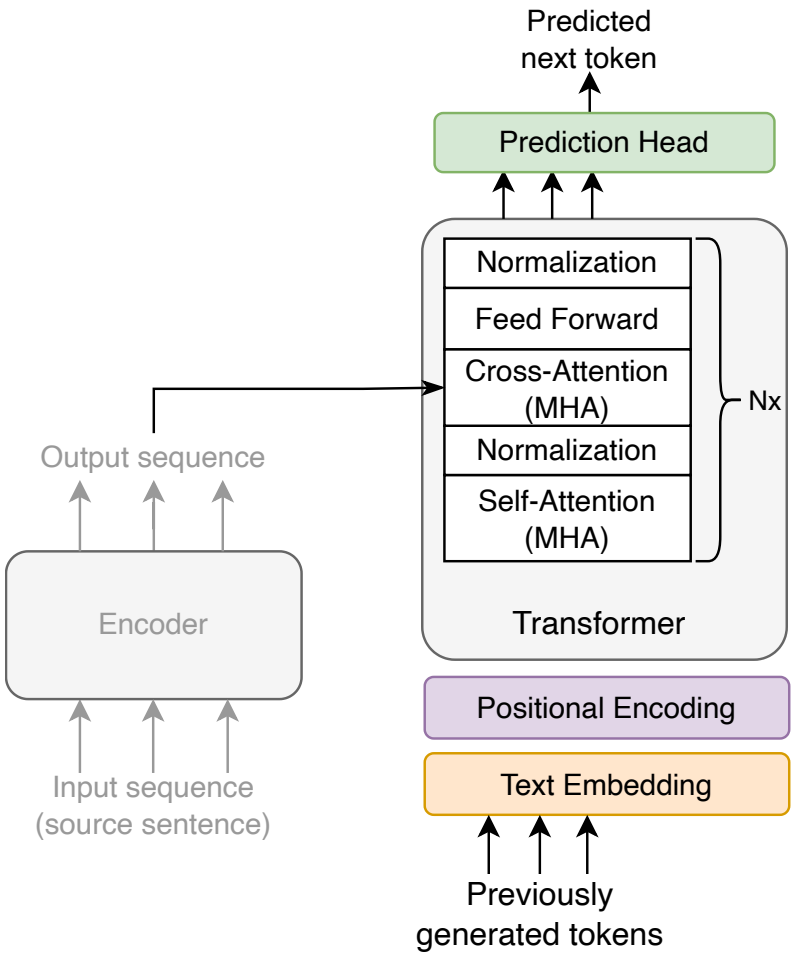
Figure 14: Decoder components
