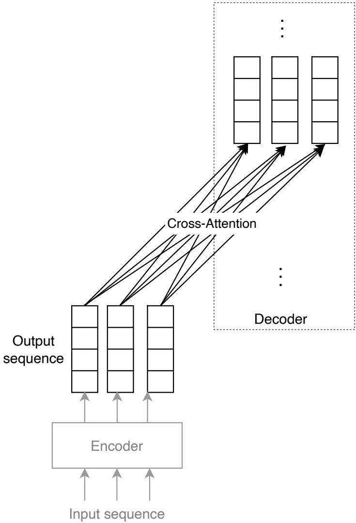
Figure 15: Cross-attention layer
